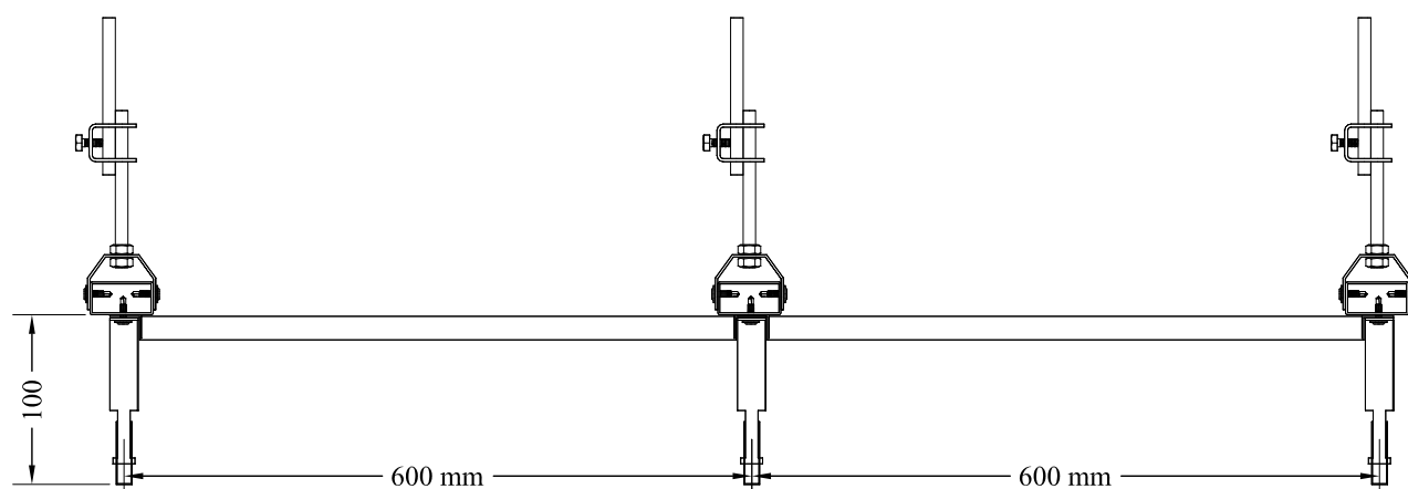
DETAIL "C-C"
