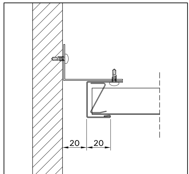
Profile W3
